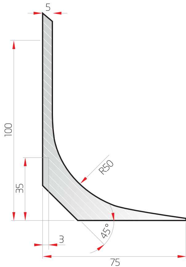
InstaCove 100 mm High
