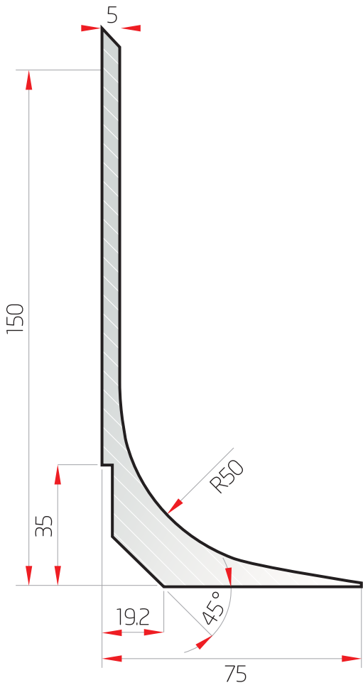
InstaCove 150mm High 50mm Radius
