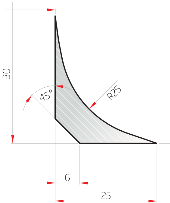
InstaCove 30mm High 25mm Radius
