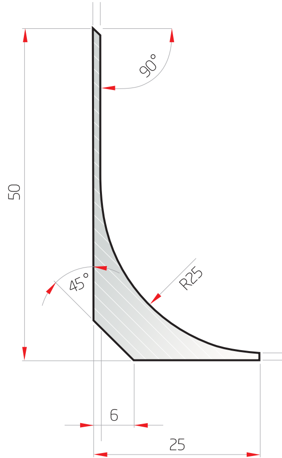
InstaCove 50mm High 25mm Radius
